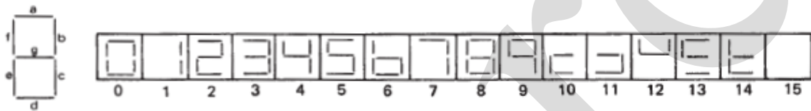
Figure 3. Segment identification
